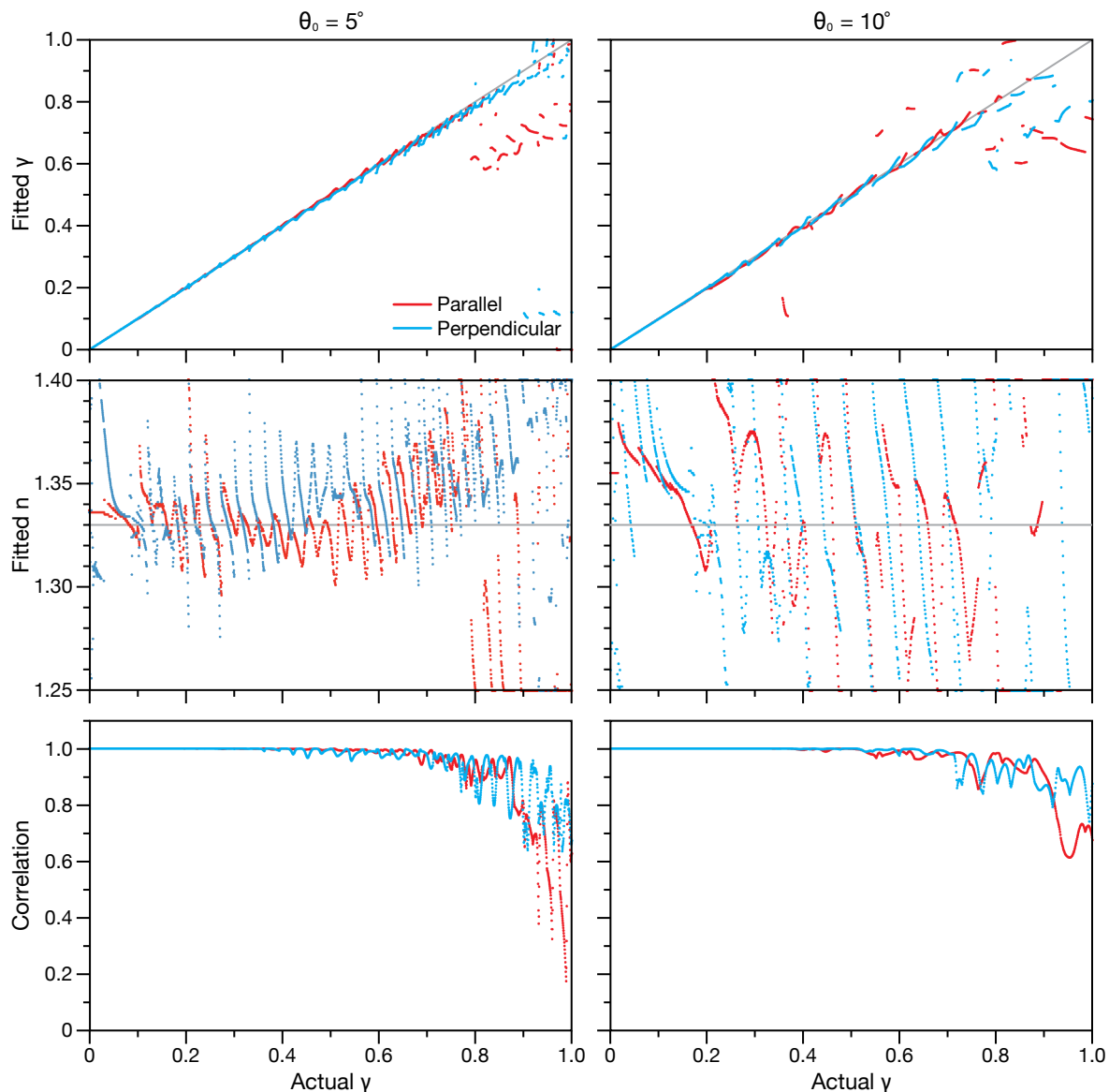
Figure 6: Best fits for angular scattering from a sphere in a Bessel beam with \theta_0 = 5^\circ and \theta_0 = 10^\circ using plane wave scattering. The range of \theta used during calculations was 70 to 110^\circ . The method for generating angular scattering plots is identical to that which is described in the caption of Fig. 5. Best-fits were found using plane wave scattering and by varying a and n until c was maximized. For presentation here, all a are converted to \gamma . Fittings were performed for both parallel and perpendicular polarization. The search space for n was restricted between 1.25 and 1.40 . Grey lines are drawn to guide the eye to where the points should fall if the fitted values match the actual values.
