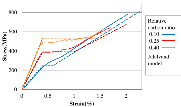
Fig. 14. Representative stress–strain curves of high modulus carbon/E-glass hybrid composites with 0.1, 0.25 and 0.4 relative carbon ratio with predicted curves. (For interpretation of the references to colour in this figure legend, the reader is referred to the web version of this article.)
