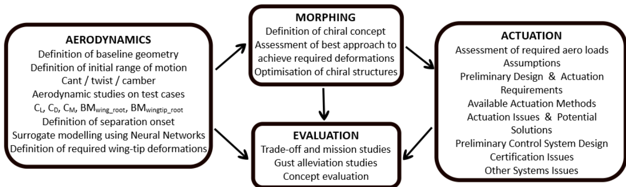
Figure 1. CLAReT Roadmap
