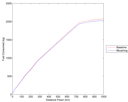
Figure 15 Fuel Consumption over Distance Flown
