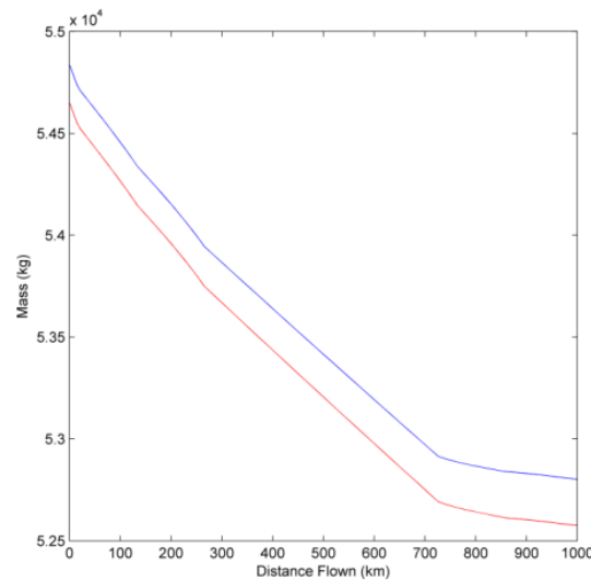
Figure 13 Mass vs. Distance Flown
