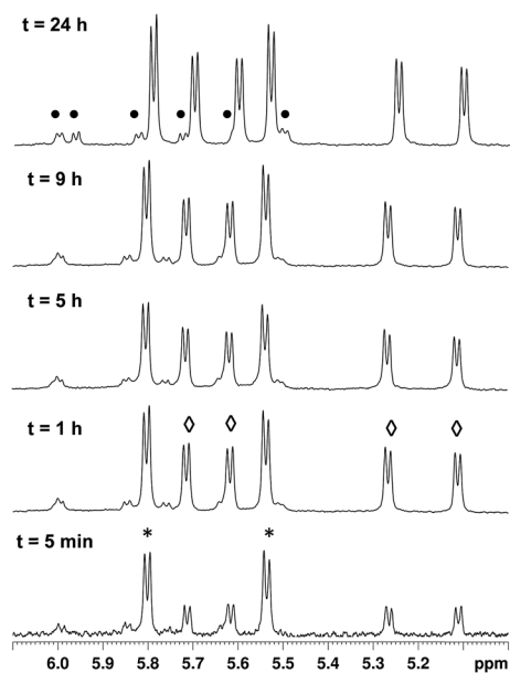
Fig. 2 The p -cymene ring proton region of the ^1\text{H-NMR} spectrum of [(\eta^6\text{-}p\text{-MeC}_6\text{H}_4\text{Pr}^i)_2\text{Ru}_2\text{Cl}_2(\mu\text{-Cl})(\mu\text{-S-}m\text{-}9\text{-B}_{10}\text{C}_2\text{H}_{11})] ( 1 ) dissolved in \text{D}_2\text{O}/\text{acetone-d}_6 (ratio 7 : 3), recorded between t = 5 min and t = 24 h at 37 °C and at pD 7. The labels correspond to p -cymene ligands in different species present in solution. The species labeled * corresponds to complex 1 , the species labeled ◇ is presumably the fully hydrolysed species [(\eta^6\text{-}p\text{-MeC}_6\text{H}_4\text{Pr}^i)_2\text{Ru}_2(\text{OD})_2(\mu\text{-OD})(\mu\text{-S-}m\text{-}9\text{-B}_{10}\text{C}_2\text{H}_{11})] , while the species labeled with ● has not been further characterised.
