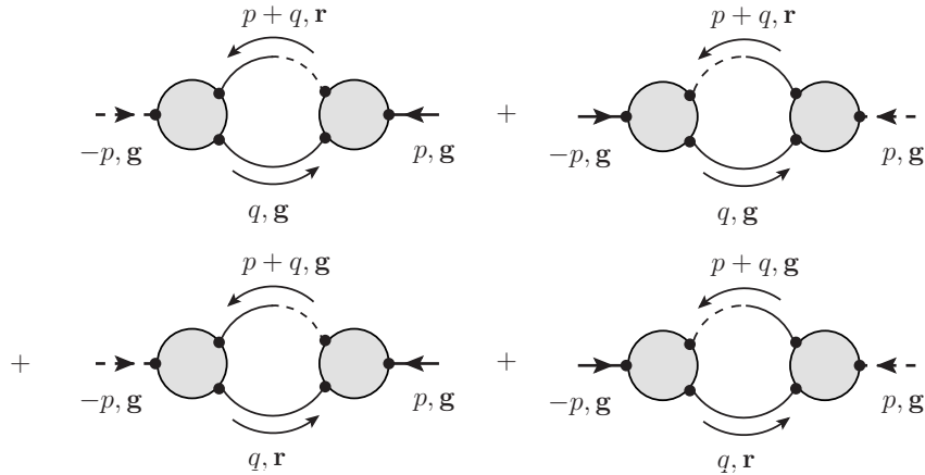
FIG. 12. Diagrams that contribute on the RHS of Eqs. (A5) – (A7). Full-dashed lines corresponds to (nonperturbative) retarded/advanced propagators G^{R/A} , while the full lines denote statistical propagators F . Full/dashed external legs denote \phi/\tilde{\phi} -field insertions. Next to the momenta we indicate the relevant modes indicated ( \mathbf{r} : radial mode, \mathbf{g} : Goldstone mode).
