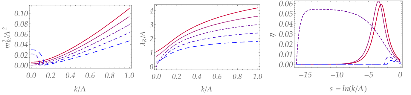
FIG. 4. N = 1 scalar model ( D = 3, T = 0 ): As we tune the (bare) quartic coupling \bar{\lambda}_\Lambda = \lambda_\Lambda/\Lambda at a fixed value of the squared field expectation value \bar{v}_\Lambda^2 = v_\Lambda^2/\Lambda = 0.078 , we observe a phase transition, when the renormalized mass m_R^2 vanishes. We define m_R^2 = \lambda_R v_R^2 in the symmetry broken regime and v_R^2 = k\bar{v}^2 , \lambda_R = k\bar{\lambda} . This is shown in the left panel where we follow the RG flow of m_R^2 as the bare coupling \bar{\lambda}_\Lambda is tuned through its critical value \bar{\lambda}_{\Lambda,cr} . In the middle panel we display the scale dependence of the renormalized coupling. At the quantum critical point the correlation length \xi \equiv m_R^{-1} diverges and the theory exhibits scaling. This scaling at the QCP is governed by the IR stable Wilson-Fisher fixed point, for which we determine the scaling exponents \eta \simeq 0.055 and z = 1 . The scale dependence of the anomalous dimension is shown in the right panel. If \bar{\lambda}_\Lambda = \bar{\lambda}_{\Lambda,cr} the anomalous dimension assumes a constant value in the scaling regime ( k \rightarrow 0 ).
