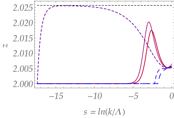
FIG. 9. N = 1 scalar model ( d = 3 , T_\Lambda > 0 ): As we tune the temperature T_\Lambda through its critical value T_{\Lambda,cr} at fixed values of \bar{v}_\Lambda^2 = v_\Lambda^2/\Lambda = 0.078 and \bar{\lambda}_\Lambda = \lambda_\Lambda/\Lambda = 1 , we observe a phase transition, where the theory exhibits scaling. We show the scale dependence of the dynamic scaling exponent z = 2 - \eta^\perp + \eta^\Omega and find z \simeq 2.025 in the scaling regime.
