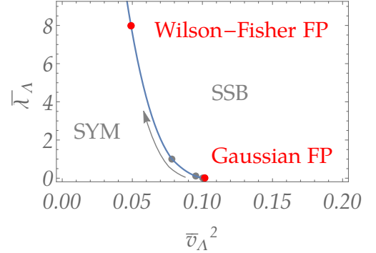
FIG. 6. N = 1 scalar model ( D = 3, T = 0 ): The crossover scale k_* that separates the canonical from the nontrivial scaling region is set by the quartic coupling at the cutoff scale \Lambda . There is a one-to-one correspondence between the scale k_* (upper panel) to points that lie on the curve connecting the Gaussian FP with the Wilson-Fisher FP (lower panel). As we move along the phase boundary (indicated by the arrow), separating the spontaneous symmetry broken phase (SSB) from the symmetric phase (SYM), towards the Wilson-Fisher FP the crossover scale is shifted to the left (upper panel). Here, the maximum correlation length \xi \equiv m_R^{-1} takes a finite value since both the bare values of the coupling \bar{\lambda}_\Lambda and field expectation value \bar{v}_\Lambda^2 have not been tuned perfectly to the phase separation line.
