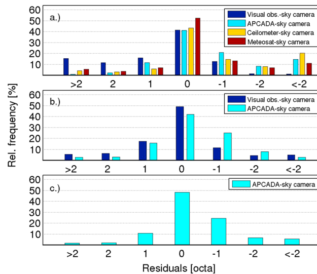
Figure 4. Relative frequency of total cloud cover differences between various techniques at (a) Payerne, (b) Jungfrauoch, and (c) Davos. Total number of compared outputs for Payerne is 2853, 7714, 6723, and 7947 for the sky camera-human observer, sky camera-APCADA, sky camera-ceilometer, and sky camera-Meteosat intercomparison, respectively. The data set from Jungfrauoch contains 1334 and 1293 observations for the sky camera-human observer and sky camera-APCADA intercomparison, respectively. For the Davos intercomparison, 5806 outputs from the sky camera and from APCADA have been compared.
