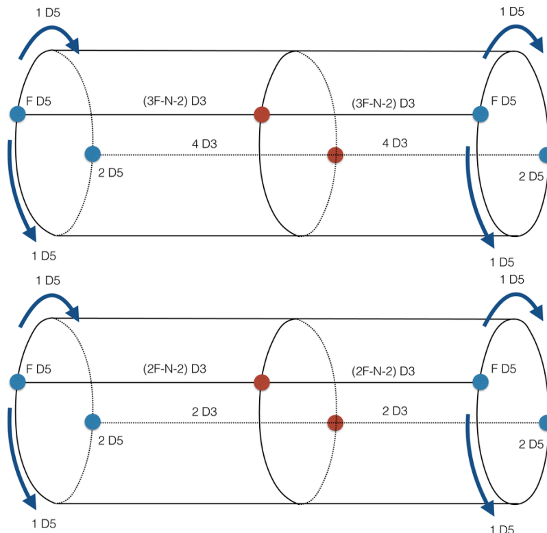
Figure 13. Aharony-like duality for models with antisymmetric matter.
