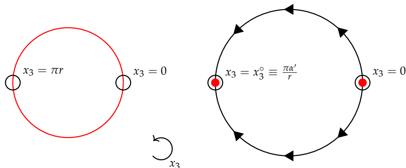
Figure 1. Geometry of the compact direction. The possible orientifolds are depicted in red color. L.h.s.: type IIA circle of radius r . R.h.s.: T-dual circle of radius \alpha'/r . The black arrowheads indicate the motion of the D-branes to the mirror point x_3 = x_3^o \equiv \pi\alpha'/r .
