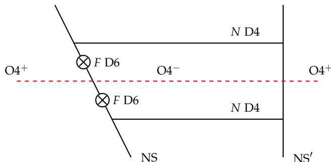
Figure 3. Brane cartoon for the realization of an \text{Sp}(2N) theory in the electric phase with an \text{O4} -plane.
