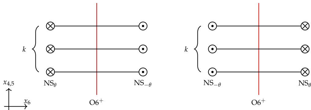
Figure 8. Electric and magnetic sides of the duality for \text{Sp}(2N) gauge theories with antisymmetric matter.
