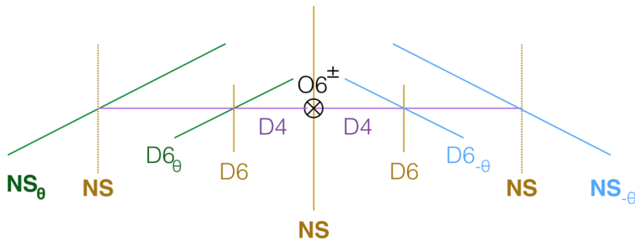
Figure 10. Brane cartoon summarizing all the constructions of unitary gauge theories with tensor matter.
