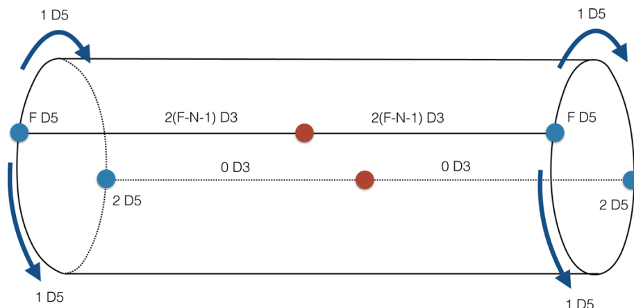
Figure 7. Aharony flow Sp in O5 picture.
