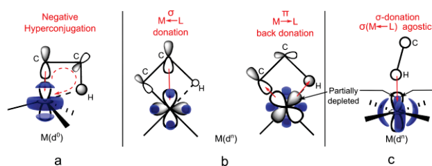
Figure 4. Three different types of agostic interactions in d^0 and d^1 transition metal complexes and their relevant molecular orbital contribution which are directly linked with the L(\mathbf{r}) pattern (blue envelope maps) at the central transition metal atoms (see also ref 17b).
