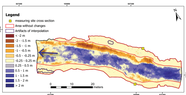
Figure 9. Channel changes after flooding of 23 August 2011 in the lower scan region. With the two yellow rectangles measurement sites of the cross section P1 are marked. Blue colours indicate deposition, red colours indicate erosion. No changes are detected in the light ochre areas.
