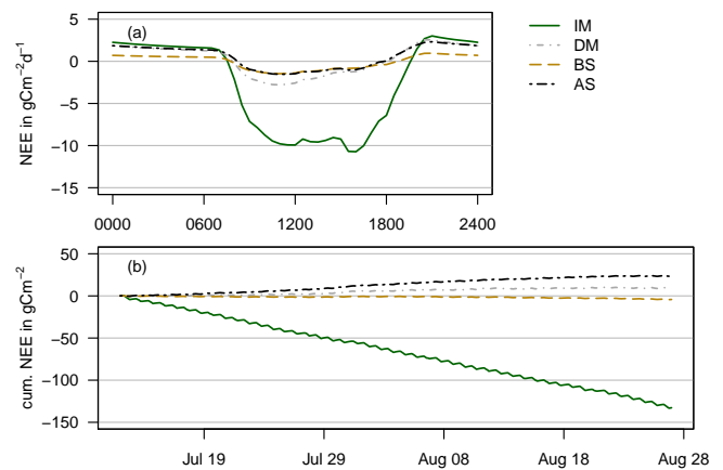
Figure 6. Model results of net ecosystem exchange (NEE) over 46 days of July and August 2012 at Kema. (a): mean diurnal cycle, and (b): cumulative NEE. The four lines represent different stages of vegetation degradation (IM, DM, BS, and AS).
