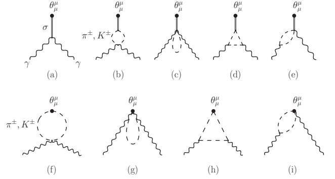
FIG. 8: Lowest order contributions to \langle \gamma_1, \gamma_2 | \tilde{\theta}_\mu^\mu(0) | \text{vac} \rangle in \chi\text{PT}_\sigma . Diagram (a) represents the contact term proportional to g_{\sigma\gamma\gamma} , while diagrams (d), (e), (h), and (i) are each accompanied by an additional crossed amplitude (not shown). Similar loop diagrams have been considered in \chi\text{PT}_3 for K_S \rightarrow \gamma\gamma [33], K_L \rightarrow \pi^0\gamma\gamma [53], and \gamma\gamma \rightarrow \pi^0\pi^0 [55, 56].
