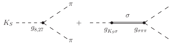
FIG. 2: Tree diagrams in the effective theory \chi\text{PT}_\sigma for the decay K_S \rightarrow \pi\pi . The vertex amplitudes due to 8 and 27 contact couplings g_8 and g_{27} are dominated by the \sigma/f_0 pole amplitude. The magnitude of g_{K_S\sigma} is found by applying \chi\text{PT}_\sigma to K_S \rightarrow \gamma\gamma and \gamma\gamma \rightarrow \pi\pi .
