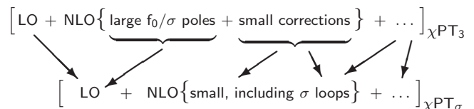
FIG. 7: Comparison of \chi\text{PT}_3 and \chi\text{PT}_\sigma . The f_0/\sigma pole terms responsible for the poor convergence of \chi\text{PT}_3 are transferred to LO in \chi\text{PT}_\sigma , where they do not upset convergence.
