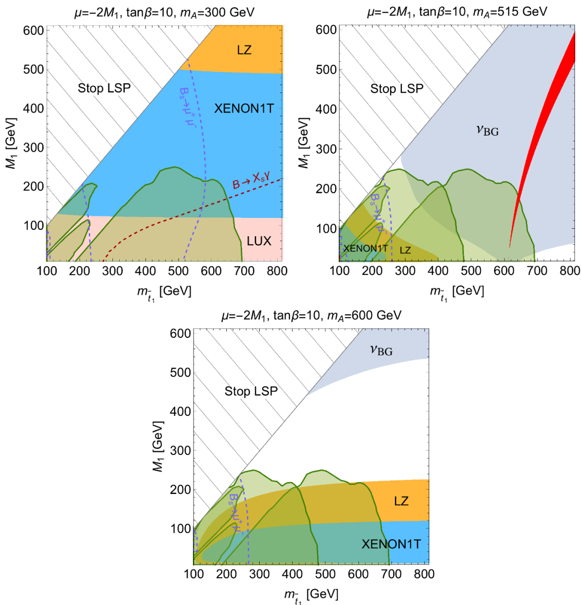
Figure 14. Current and projected limits in the (m_{\tilde{t}_1}, M_1) plane from h, H and \tilde{t}_{1,2}, \tilde{b}_L exchange in \chi -xenon scattering. The three plots represent different values of m_A , for fixed \tan\beta = 10 . For A_t^{\max} < 0 , the regions between the purple dashed lines are excluded by B_s \rightarrow \mu^+ \mu^- , while regions to the left of the dark red dashed lines are excluded by B \rightarrow X_s \gamma . Excluded regions from direct detection are color-coded as in figure 13.
