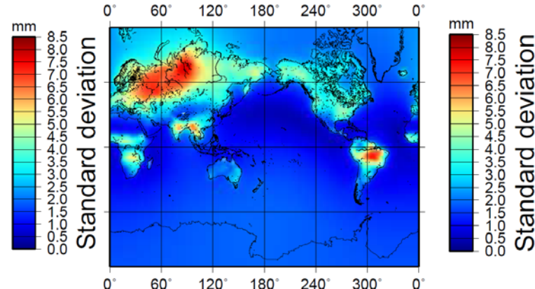
CWSL (after detrend)
