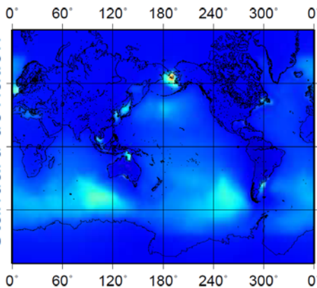
NTOL (after detrend)
