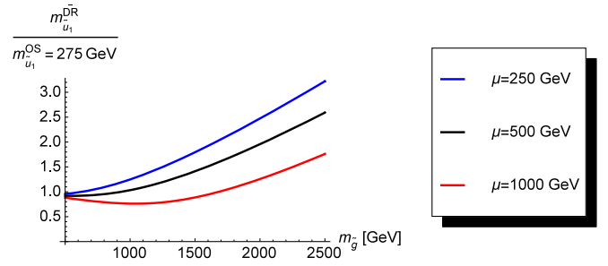
FIG. 5 (color online). Ratio of the \overline{\text{DR}} stop mass over its on-shell mass for m_{u_1}^{\text{OS}} = 275 GeV as generated by Eq. (48) and A^t = 1 TeV as a function of the gluino mass for different values of the renormalization scale \mu (see text).
