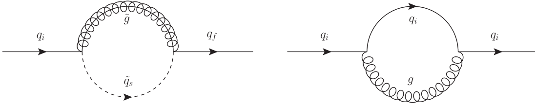
FIG. 1. Quark self-energy diagrams.
