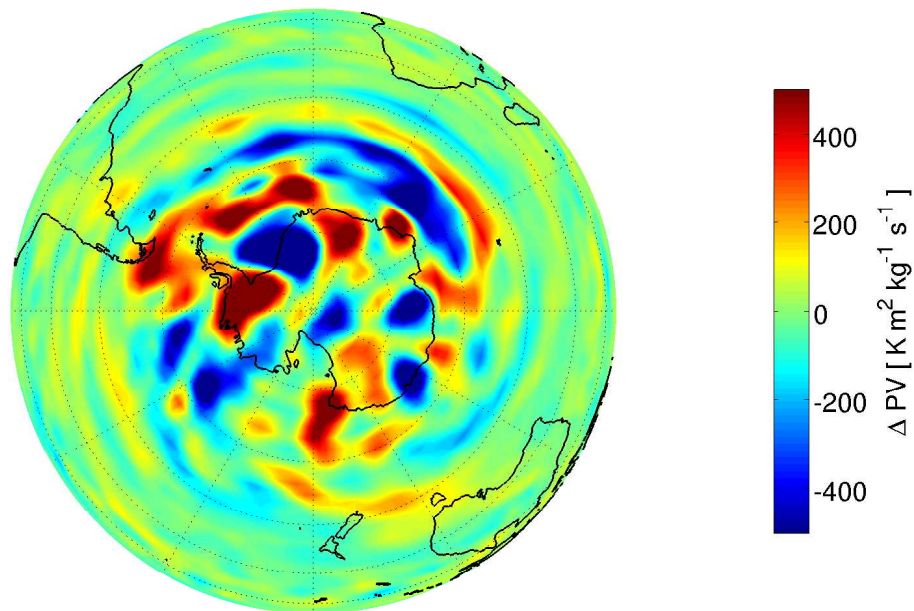
Figure 10. Difference of potential vorticity from 18:00 to 06:00 UT derived from the ERA-Interim reanalysis for 21 June 2012 in the Southern Hemisphere at 5 hPa.
