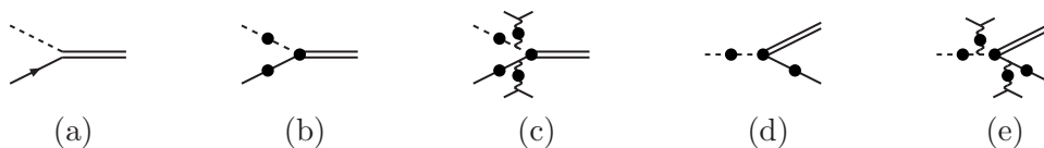
Figure 2. Examples of processes for right-handed neutrino production: (a) a tree-level process producing a massive right-handed neutrino (double line) out of a coalescence of a Higgs (dashed line) and a left-handed lepton (solid line); (b) the same process after HTL resummation, generating thermal self-energies or effective vertices (filled blobs); (c) processes contributing at the same order as (b), due to exchanges of soft W^\pm, Z^0, \gamma bosons; (d) another channel allowed by the thermal masses generated by HTL resummation (if m_\phi > M ); (e) processes contributing at the same order as (d). In the language of eq. (4.5), the processes (a)–(c) originate from the range k_0 = \omega_1 + \omega_2 , \omega_1 > 0 , \omega_2 > 0 , whereas (d) and (e) correspond to \omega_2 = k_0 - \omega_1 , \omega_1 < 0 , where \omega_1 is the lepton, \omega_2 the Higgs, and k_0 the right-handed neutrino energy.
