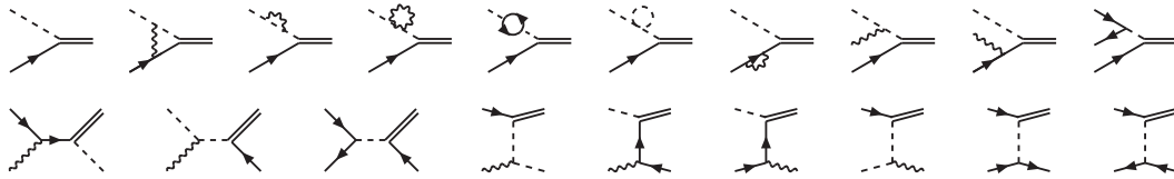
Figure 1. The processes, up to O(g^2) , through which right-handed neutrinos can be generated. Arrowed, dashed, and wiggly lines correspond to Standard Model fermions, scalars, and gauge fields, respectively, whereas right-handed neutrinos are denoted by a double line. The closed “virtual” loops include both vacuum and thermal corrections.
