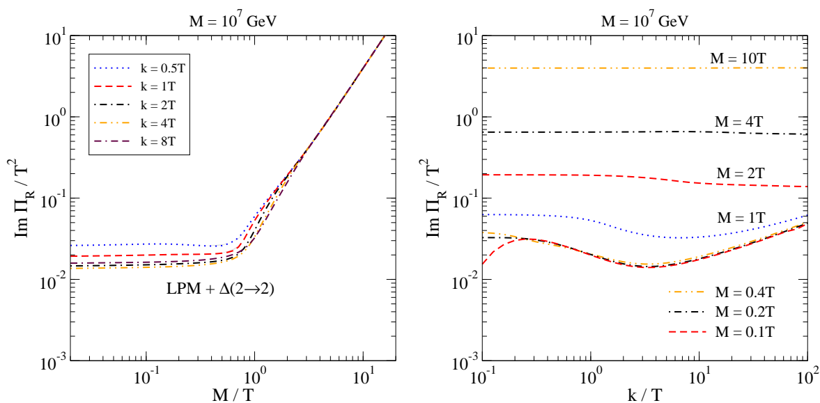
Figure 4. Left: final results for the correlator in eq. (7.2). Right: the same results as a function of k/T . The couplings and the renormalization scale are fixed as specified in appendix D.
