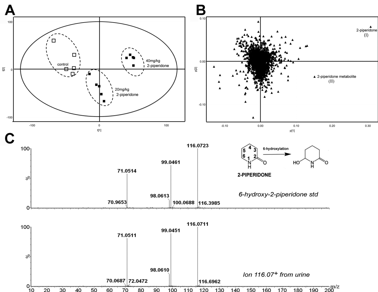
FIG. 5. Identification of 6-hydroxy-2-piperidone as a 2-piperidone metabolite. (A) Separation of control WT ( \square ) mice from the WT mice ( \blacksquare ) treated with 20 and 40 mg/kg of 2-piperidone in the scores plot of a PLS-DA model on the urine metabolomes. (B) Identification of 2-piperidone (I) and 2-piperidone metabolite (II) in the loadings plot. (C) A comparison of MS/MS spectra of urinary 2-piperidone metabolite ( [M + H]^+ = 116.07\ m/z ) and synthesized 6-hydroxy-2-piperidone standard.
