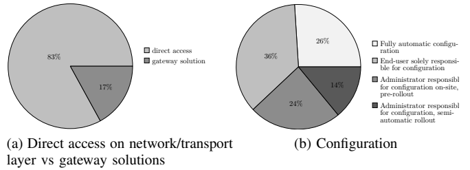
Fig. 5. Enterprise integration
