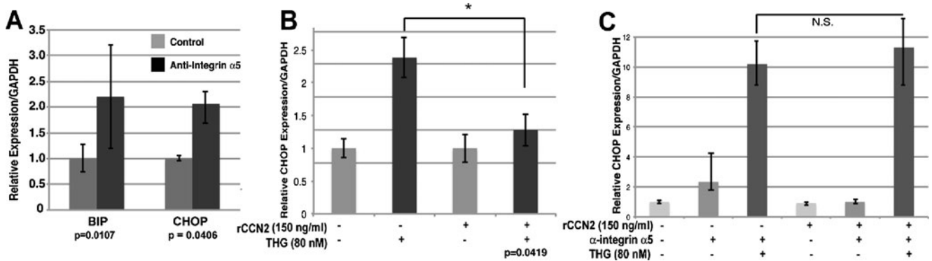
Fig. 5 Blocking Integrin \alpha 5 results in chondrocyte stress. Primary sternal chondrocytes were serum starved and treated with anti-integrin \alpha 5 blocking antibody or goat serum (control) for 24 h, after which BiP and CHOP mRNA levels were quantitated by qRT-PCR and normalized to GAPDH. BiP and CHOP expression were increased by
