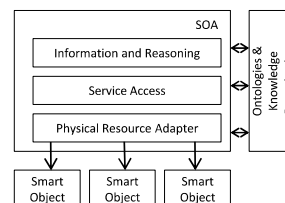
Fig. 1. Layered Architecture
