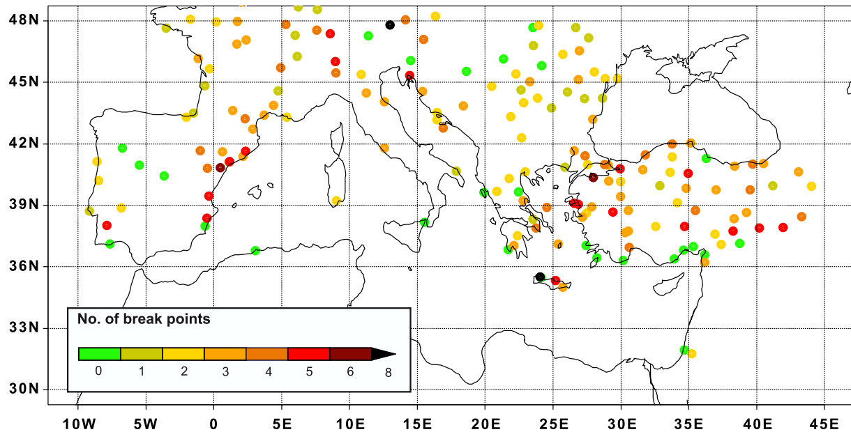
Figure 9. The number of breakpoints detected for each series indicated by color.
