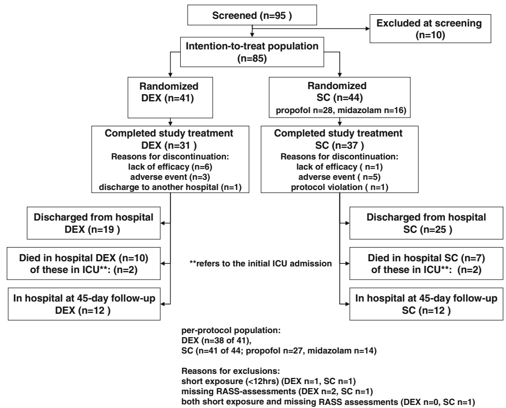
Fig. 2 Randomization, completion of study treatment, reasons for discontinuation of study treatment, and patient outcomes in intention-to-treat population; inclusions into per-protocol population and reasons for exclusions. Note: one patient in each study arm was lost to follow-up after day 31; both were still hospitalized after discharge to another hospital, and were considered as being in hospital at 45-day follow-up
