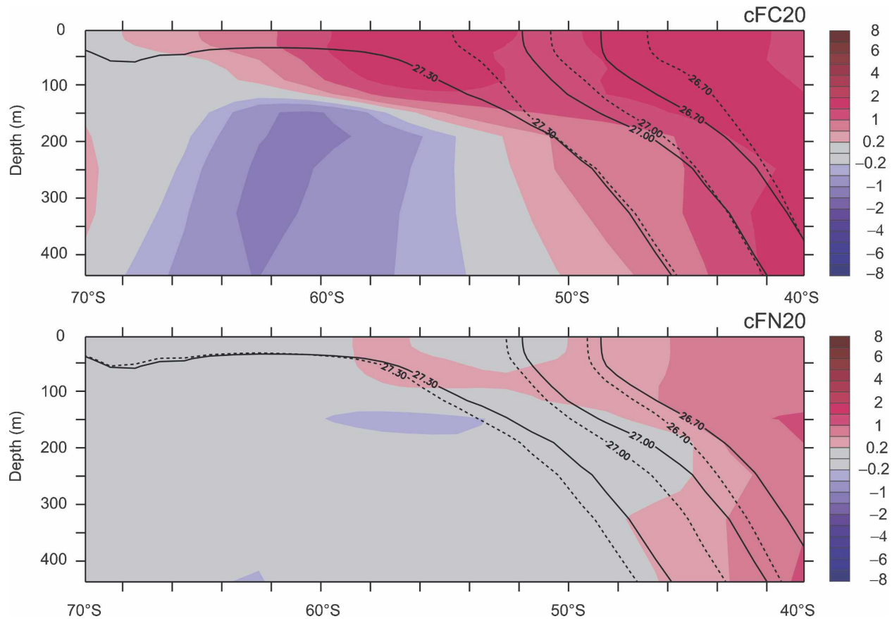
FIG. 5. Zonally averaged changes in temperature in K (colors) and zonally averaged isopycnals in \text{kg m}^{-3} – 1000 \text{ kg m}^{-3} (contours) in the sector from 0^\circ to 60^\circ\text{E} coinciding with the area of major warming in the Southern Ocean (see Fig. 2b). Shown are changes between control and means over 10 yr starting at year 100 for experiments (top) cFC20 and (bottom) cFN20. Isopycnals are shown for the control simulation (solid) and the mean over 10 yr starting at year 100 (dashed). In cFC20 the isopycnals move equatorward, whereas for cFN20 they move poleward.
