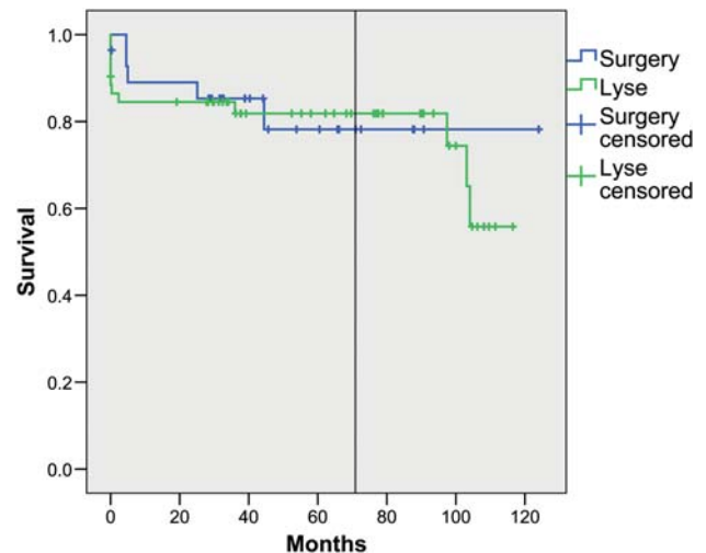
Figure 1: Kaplan-Meier survival.
