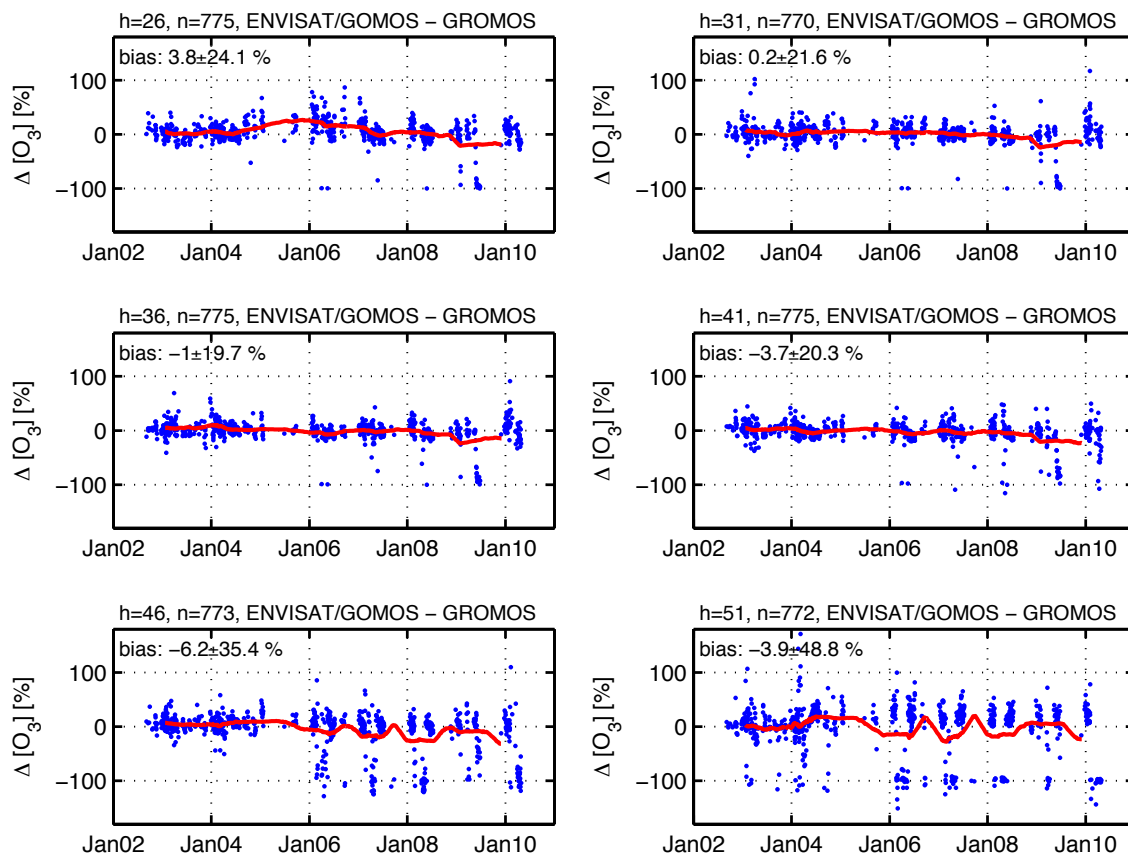
Fig. 7. Time series of the relative difference \Delta\text{O}_3 of the ozone concentration profiles of GOMOS and the ground-based microwave radiometer GROMOS at altitudes h = 26, 31, 36, 41, 46 , and 51 km. The red line is a moving average over 80 blue dots. Sometimes GOMOS fails to detect ozone at upper altitudes (more frequently at h = 46 and 51 km with \Delta\text{O}_3 values close to -100\% ). N corresponds to the number of collocations.
