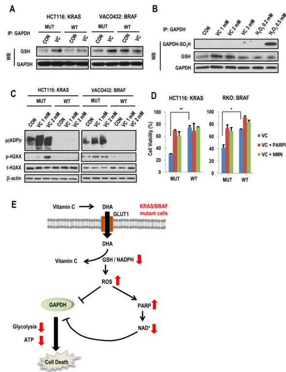
Fig. 4. Vitamin C-induced ROS inhibits GAPDH by cysteine S-glutathionylation and depleting \text{NAD}^+
