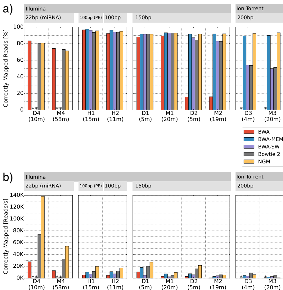
Fig. 2 Mapping accuracy and mapping efficiency for different mappers and different input data. a Percentages of correctly mapped reads; and (b) number of correctly mapped reads per second for five mappers. Table 1 gives a detailed description of the data. A * indicates that at least 99.9 % of the reads were not mapped, due to limitations of the mapper. Teaser runtime in minutes is shown in parenthesis
