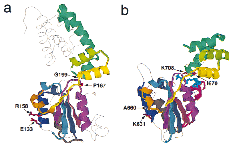
Figure 2 Core structural components corresponding to conserved regions in the AAA + multiple alignment. (a) Structural components of the DNA polymerase \delta' subunit (pdb: 1A5T). (b) Structural components of NSF-D2 (pdb: 1NSF). Four key conserved positions are indicated. (1) E133/K631 and (2) R158/A660 correspond to conserved (charged residue) positions in boxes VI and VII, respectively (see Fig. 4 and text). (3) P167/I670 corresponds to a conserved hydrophobic position in box VII' that presumably establishes an important contact with the amino-terminal region of the AAA + module (Yu et al. 1998); in both Pol III \delta' and NSF-D2 this hydrophobic residue contacts a Trp residue. (4) G199/K708 corresponds to a conserved basic residue position within the sensor-2 motif (see text). Each core structural element has the same color as the bar over the corresponding aligned region in Fig. 1. Unconserved regions are shown as single gray threads. ATP is colored cyan in b. The \beta -strand and three-helix bundle corresponding to the last four (orange, yellow, lime, and green) components and the box II (scarlet) component are distinct structural characteristics of the AAA + class (see Fig. 3 and text). Note, however, that the box II component is absent from Pol III \delta' . These and the other structural images were created using the RASMOL program by Roger Sayle (GlaxoWellcome).
