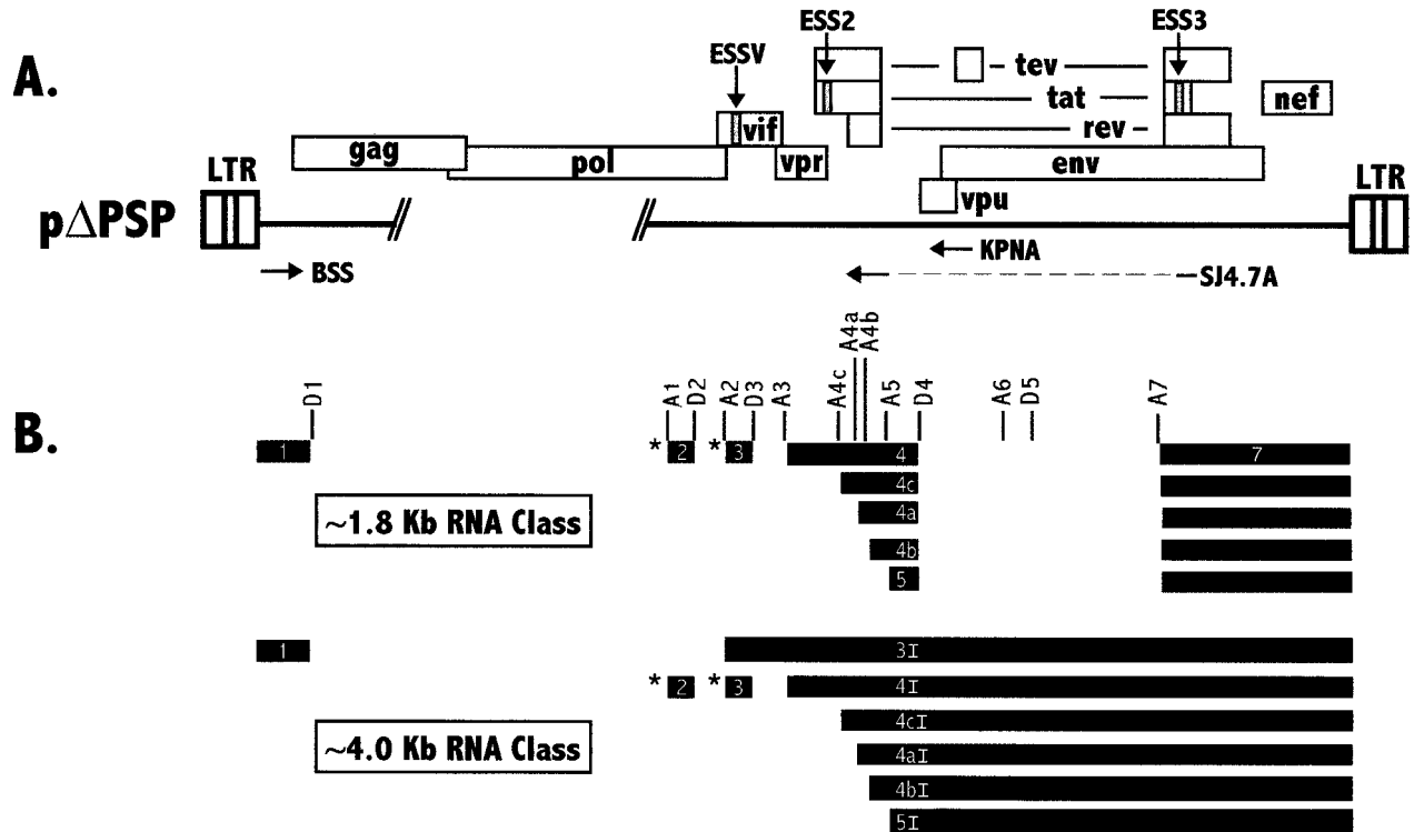
FIG. 1. (A) Structure of the HIV-1 NL4-3 genome. Boxes indicate open reading frames. Hash marks represent endpoints of gag-pol deletion in p \Delta PSP. ESS sequences are shown by shaded boxes. Oligonucleotide primers used are indicated by arrows designating position and orientation. LTR, long terminal repeat. (B) Structures of the small ( \sim 1.8-kb) and intermediate ( \sim 4.0-kb) size classes of HIV-1 transcripts. Exons are indicated as black bars. The exons within the different RNA species are designated by numbers (and sometimes letters) within the boxes according to the nomenclature of Purcell and Martin (35). The exon designations with the letter I indicate exons present only in the intermediate-size HIV-1 mRNA species. The alternative noncoding exons 2 and 3 are indicated with asterisks. Locations of 5' (D) and 3' (A) splice sites are shown.
