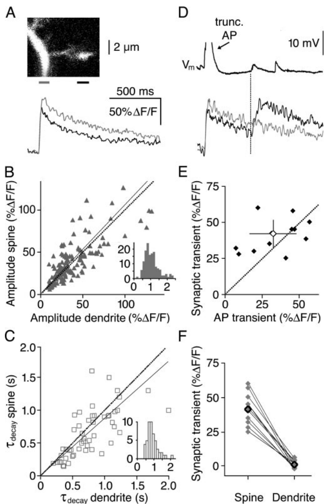
Figure 3. AP and synaptically mediated calcium transients are observed in spines. A , Spine and dendritic (\Delta F/F)_{AP} transients are similar. The scan shows a large spine/gemmuole, located at 111 \mu\text{m} from the cell soma. Below, the averaged filtered transients in dendrite (gray) and spine (black) are shown, as measured in the regions with respective colors indicated below the scan. The horizontal line scan was aligned with the spine. B , Similar (\Delta F/F)_{AP} amplitudes are observed in dendrites and spines. The scatterplot shows transient amplitudes in spines versus transient amplitudes in the adjacent dendrite. The dotted line represents the diagonal x = y , and the straight line a linear fit to the data. The inset shows a histogram of amplitude ratios spine/dendrite. C , Slightly faster (\Delta F/F)_{AP} decay is seen in spines than in dendrites. The scatterplot shows transient decay constants in spines versus transient decay time constants in the adjacent dendrite, with details similar to B . D , Spontaneous synaptic events occur. The synaptic transient shown was measured in the spine from A , with identical scaling. The top trace shows the voltage recording with truncated evoked AP and spontaneous EPSPs. The bottom shows corresponding calcium signals in the spine (black) and adjacent dendrite (gray). Note that the AP evokes a transient both in spine and dendrite, whereas the spontaneous transient is localized to the spine and coincides with a spontaneous EPSP. E , Synaptic and AP-evoked \Delta F/F amplitudes are similar. The scatterplot shows mean synaptic versus AP-evoked \Delta F/F amplitudes in each spine where spontaneous synaptic events were observed ( n = 12 ). The open diamond represents the population mean \pm SD. F , Synaptic calcium is not observed in the adjacent dendrite. The plot shows mean synaptic \Delta F/F amplitudes in all spine/dendrite pairs where spontaneous synaptic events were observed ( n = 12 ). Mean values are represented by open diamonds.
