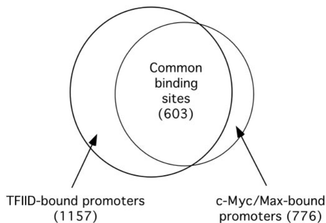
Fig. 3. c-Myc and Max colocalize with TFIIID in Burkitt's lymphoma cells. A Venn diagram compares the gene promoters bound by the c-Myc/Max complexes and that by TFIIID in Daudi cells.
