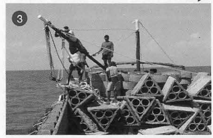
Fig.3: Deployment process of grouper modules with pulleys
