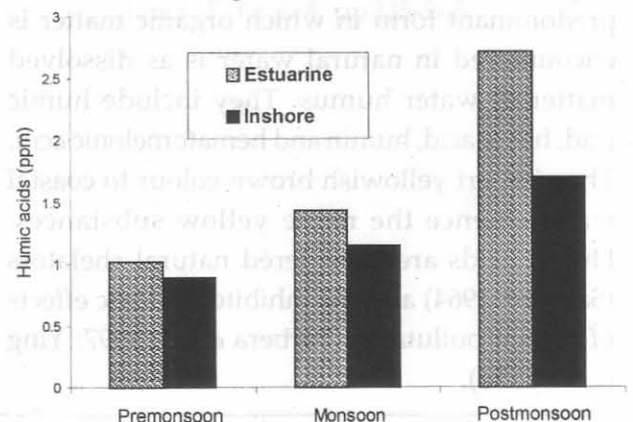
Fig. 1 Humic acids in Cochin sediments
