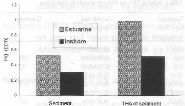
Fig. 3 Levels of Hg in sediment and in THA extracted from the sediment
