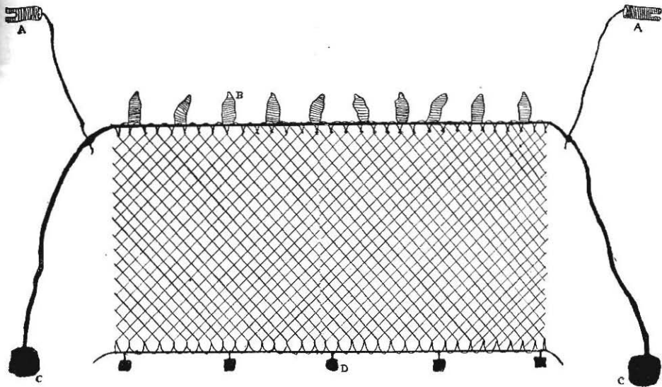
TEXT-FIG. 2. Diagrammatic sketch of Kanthabale operated along Mangalore coast. (A) Bamboo float. (B) Wooden float. (C) Stone weight. (D) Small stone weight.
