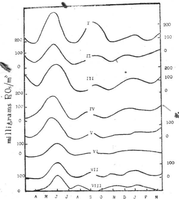
FIG. 5. Annual variation of phosphates expressed as mgm. \text{P}_2\text{O}_5/\text{m}^3 at the different stations during 1954-'55.
