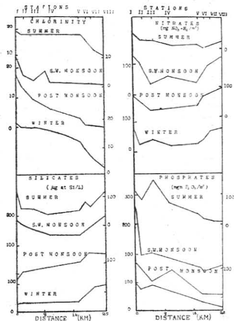
FIG. 7. Horizontal distribution of chlorinity, silicates, phosphates and nitrates in the different seasons during 1954-'55.
