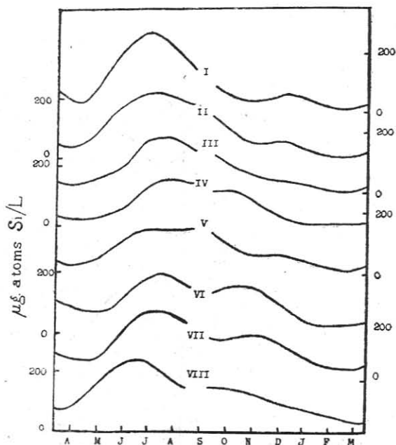
FIG. 4. Annual variation of silicates expressed as \mu\text{g at. Si/L} at the different stations during 1954-55.
