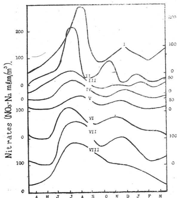
FIG. 6. Annual variation of nitrates expressed as \text{mg. NO}_3\text{-N}_2/\text{m}^3 at the different stations during 1954-'55.
