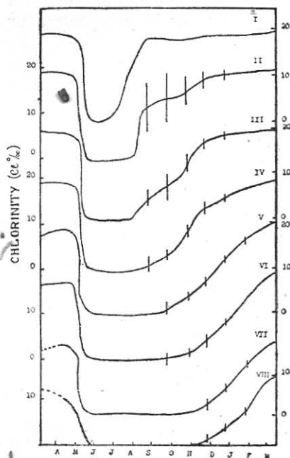
FIG. 3. Annual variation of chlorinity (Cl ‰) at different stations during 1954-55. (Bars denote average deviation.)
