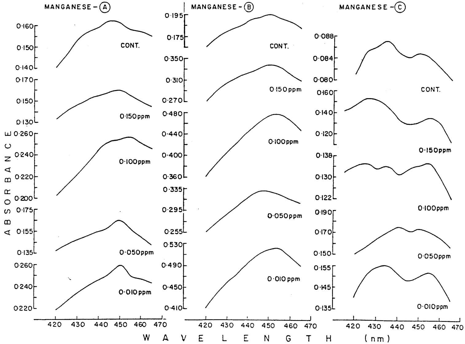
FIG. 39 ABSORPTION SPECTRA
