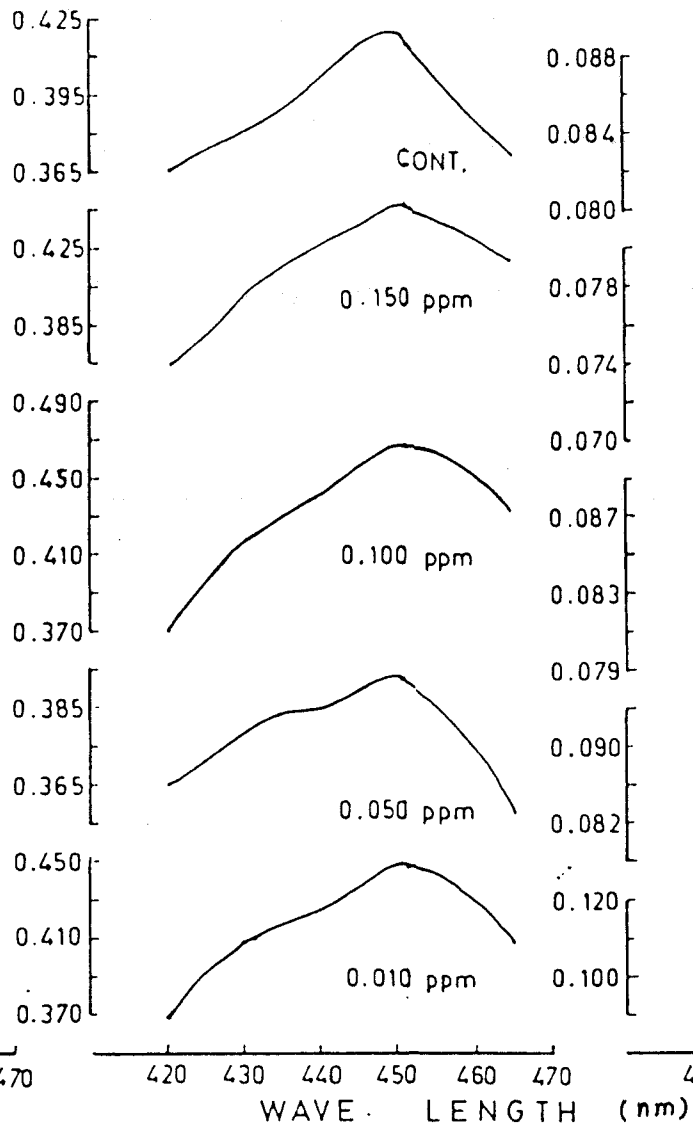
ABSORPTION SPECTRA
