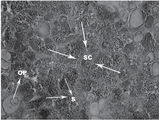
Fig. 2b. Gonadal development of juvenile after 30 weeks in presence of active adult male fish that was changing from male to female; Spermatocyte cysts (SC), Spermatids(S), few oocytes in perinucleolar stage (OP)
