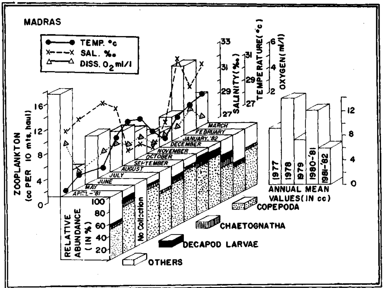
Fig. 7. Trends in secondary production at Madras.
