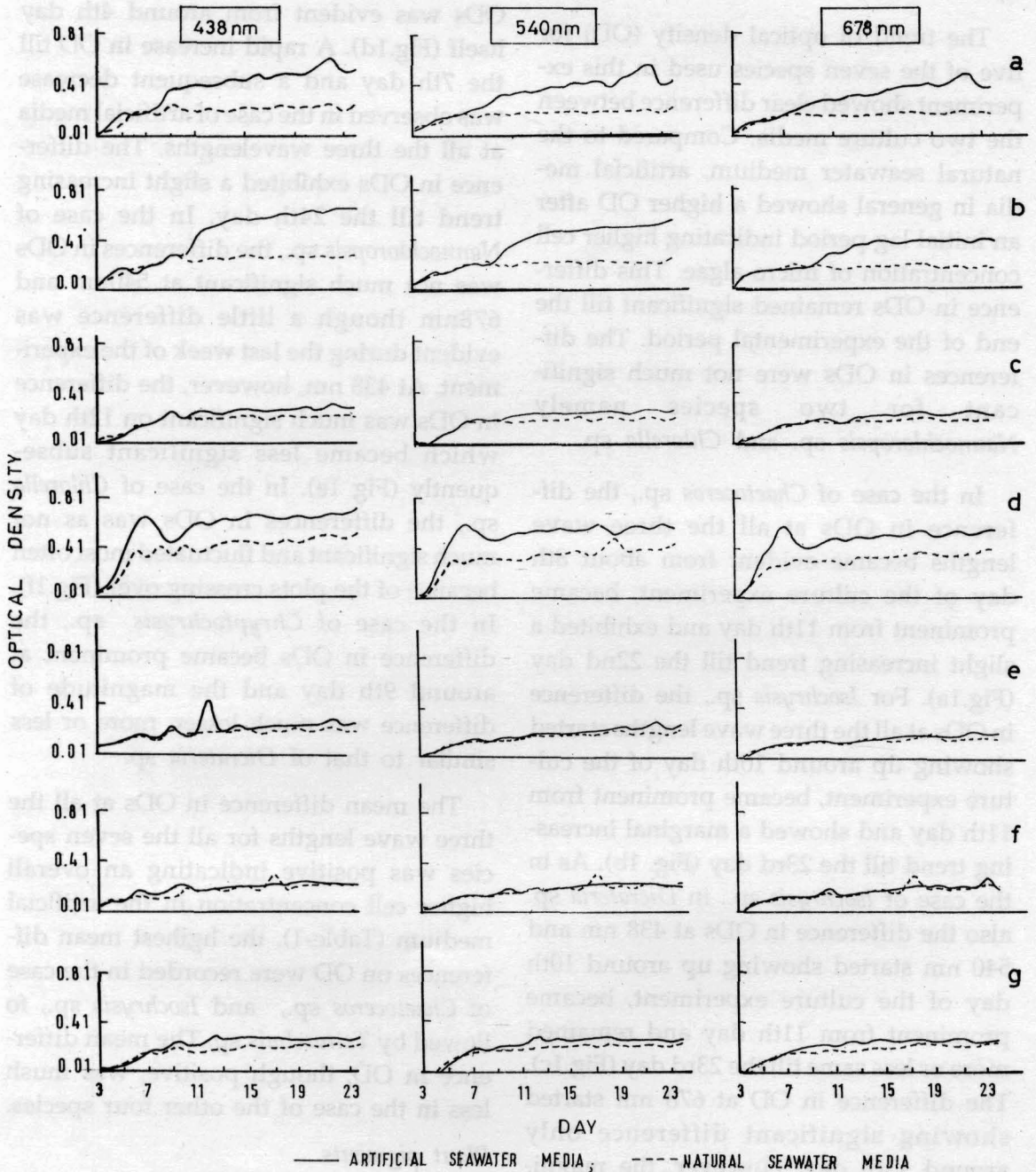
Fig. 1. The daily variation in Optical Density in the cultures in artificial medium and natural seawater medium w.r.t seven species of micro-algae (a) Chaetoceros sp., (b) Isochrysis sp., (c) Dicrateria sp., (d) Tetraselmis sp., (e) Nannochloropsis sp., (f) Chlorella sp., and (g) Chryptochrysis sp. during the experimental period.
