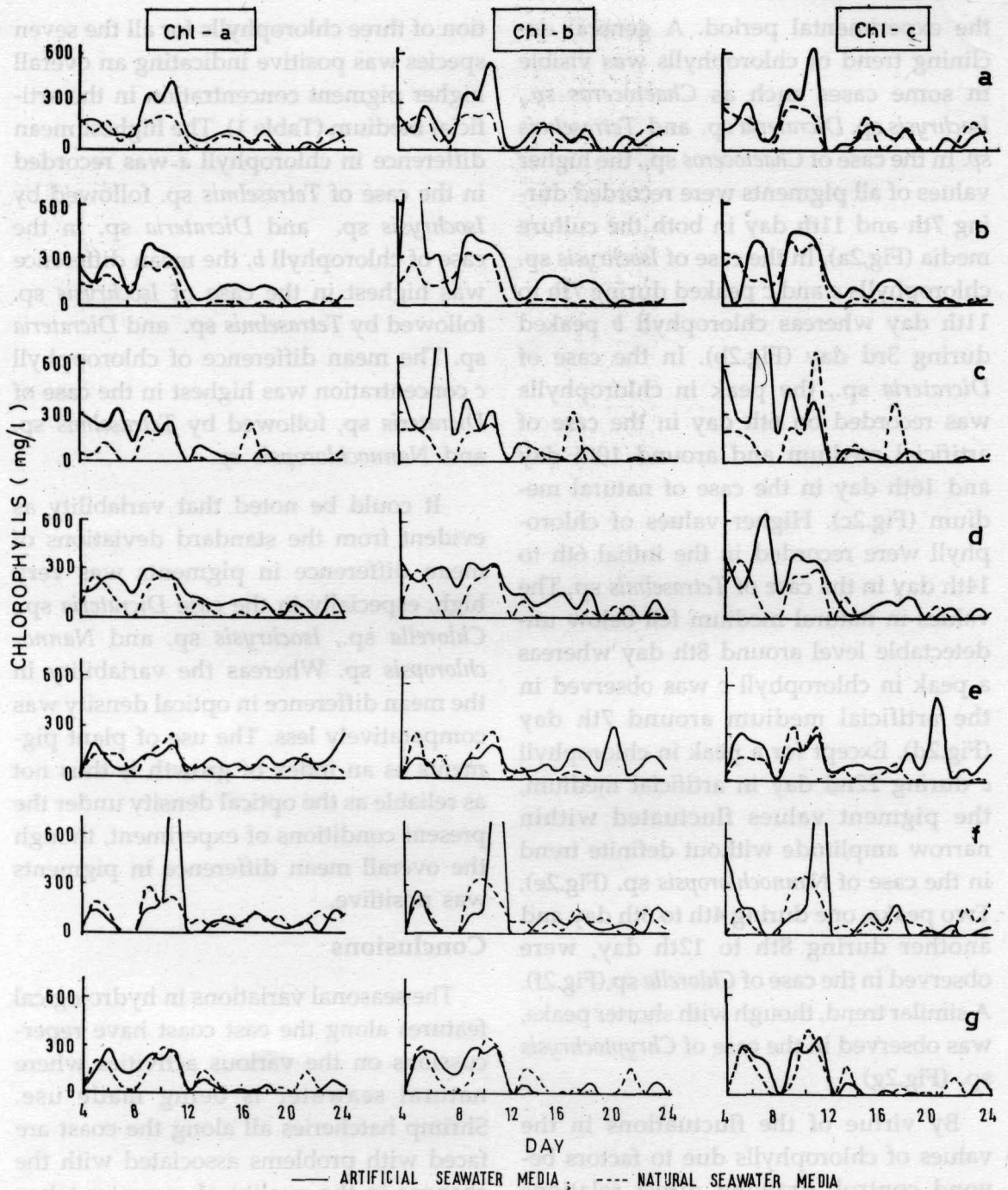
Fig. 2. The daily variation in Chlorophylls in the cultures in artificial medium and natural seawater medium w.r.t seven species of micro-algae (a) Chaetoceros sp., (b) Isochrysis sp., (c) Dicrateria sp., (d) Tetraselmis sp., (e) Nannochloropsis sp., (f) Chlorella sp., and (g) Chryptochrysis sp. during the experimental period.
