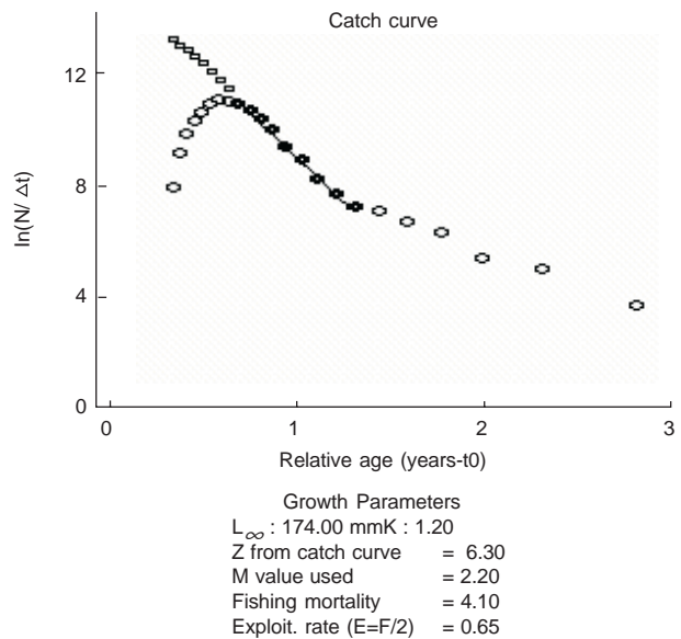
Fig. 3. Length-converted catch curve of P. pelagicus .
