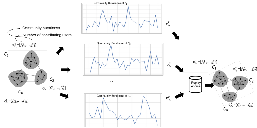
Figure 5.5: Community feature forecasting and replay framework
