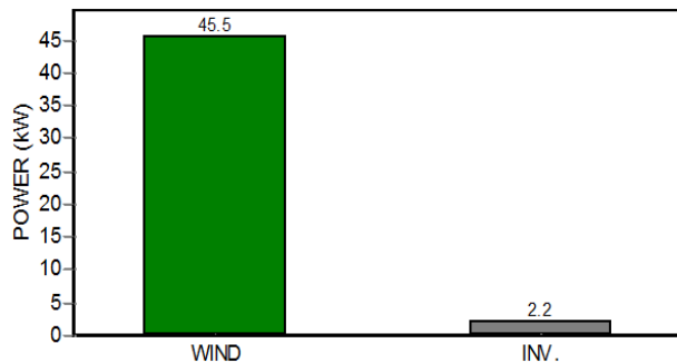
Figure 24. Optimal unit size of standalone wind system
