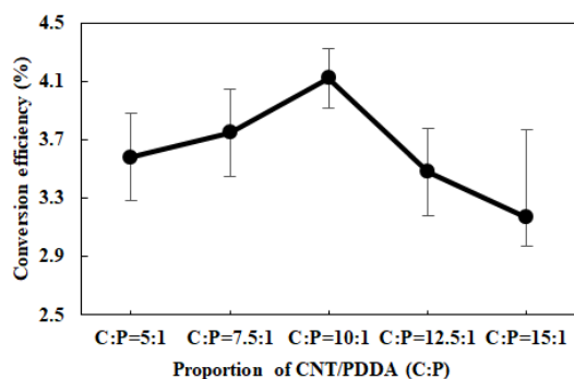
Figure 8. The conversion efficiencies of the DSSCs using CNT/PDDA counter electrodes with different CNT/PDDA ratios. Error bars represent standard deviation
