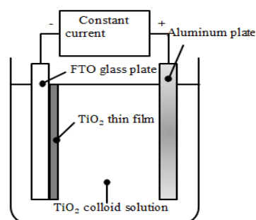
Figure 1. EPD setup for fabricating the photoanode
