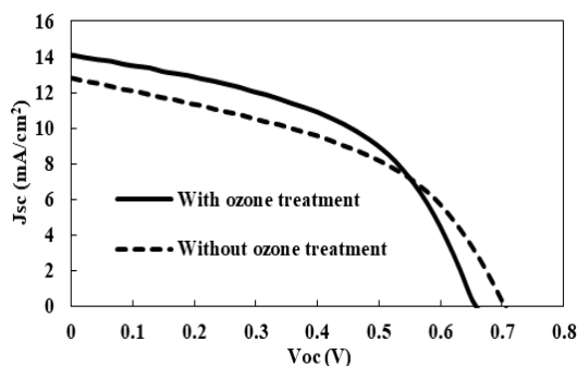
Figure 9. The J-V curves of the DSSCs using the photoanodes with and without the ozone treatment and the optimum CNT/PDDA counter electrodes (CNT/PDDA=10:1)
