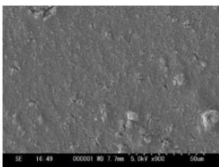
Figure 5. An SEM image of the surface of the photoanode after annealing
