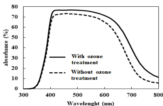
Figure 7. UV-vis absorbance spectra of the dyed photoanodes with and without the ozone treatment
