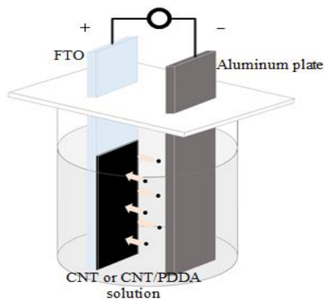
Figure 2. EPD setup for fabricating the counter electrode
