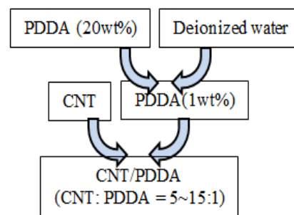
Figure 3. The preparation flow of CNT/PDDA solutions used for fabricating CNT/PDDA counter electrodes
