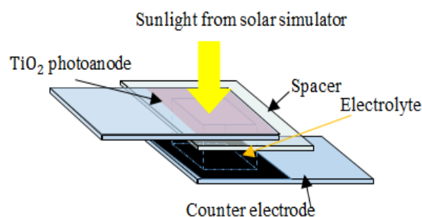
Figure 4. DSSC construction
