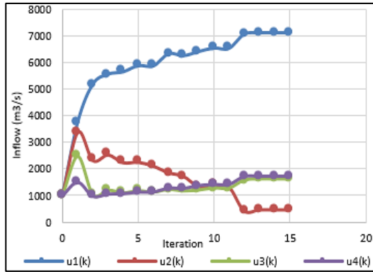
Figure 3. Control input versus iteration (case 1)
