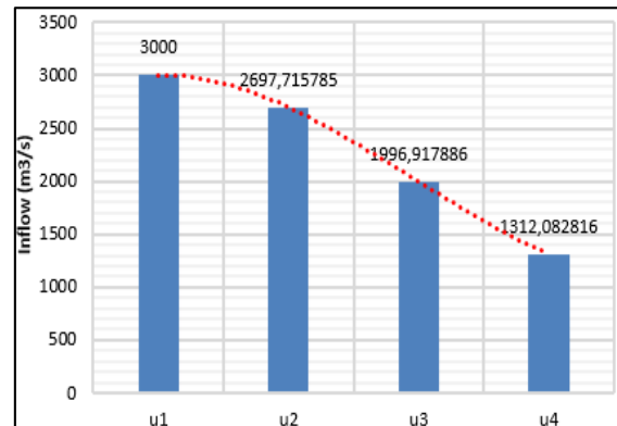
Figure 10. Optimum control (case 3)
