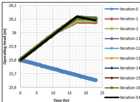
Figure 7. Reservoir head versus time (case 2)
