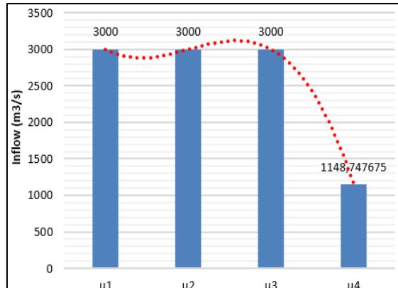
Figure 8. Optimum control (case 2)
