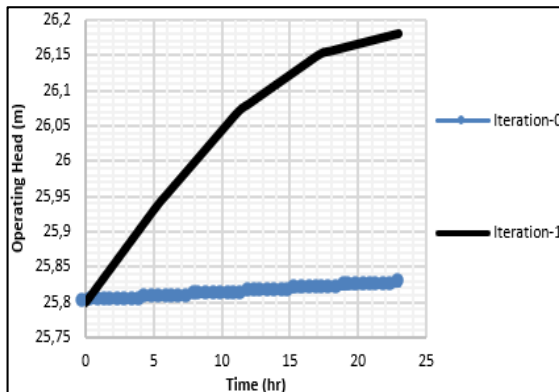
Figure 9. Reservoir head versus time (case 3)
