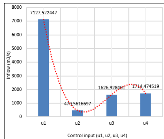
Figure 2. Optimum control (case 1)
