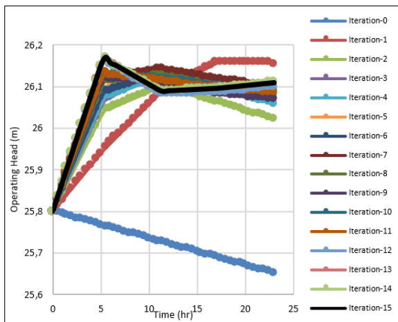
Figure 1. Reservoir head versus time (case 1)
