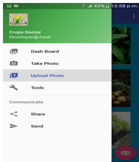
Figure 6. Menu list
