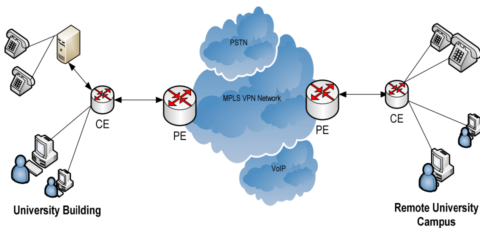
Figure 2. Proposed Architecture
