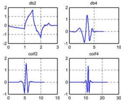
Figure 3. Four Mother wavelets functions
