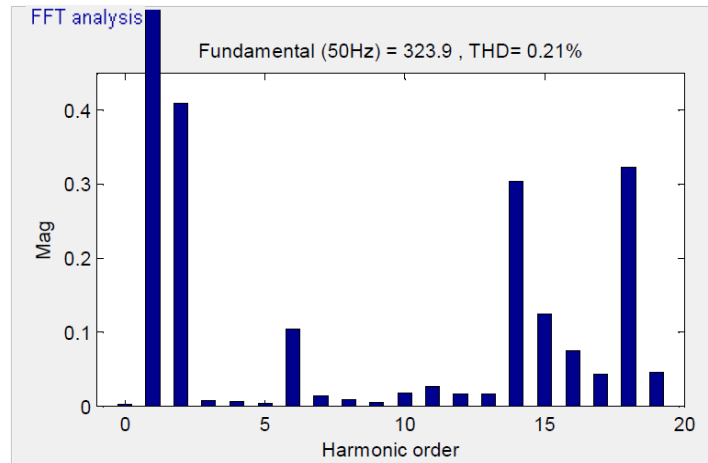
Figure 7. THD of the 9 – level MLI with R load
