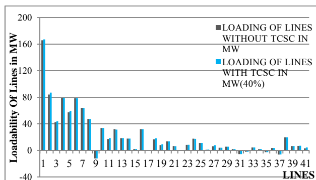
Figure 7. Loadability of Lines At 40% Compensation
