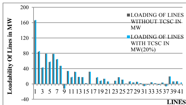
Figure 6. Loadability of Lines At 20% Compensation
