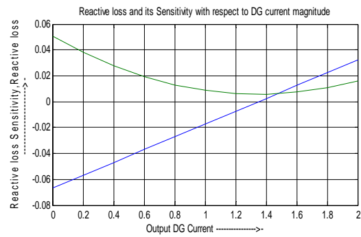
Figure 6. Reactive loss and its sensitivity with respect to DG current Magnitude
